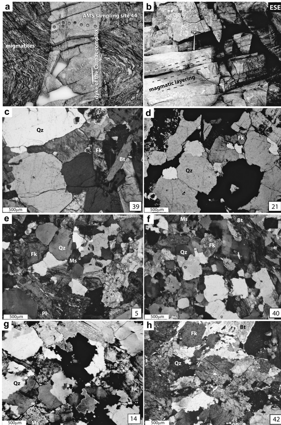
Fig. 2. Outcrop pictures of representative dykes of the Carnac Complex, and microphotographs of the magmatic microstructures. On the right bottom of the thin section pictures c–h, the numbers refer to the sample name and to the AMS sites. Their location is given on Fig. 1. The thin sections are oriented parallel to the WNW–ESE stretching. Qz: quartz; Fk: K-feldspar; Pl: plagioclase; Bt: biotite; Ms: muscovite (a) Structural relationships between a steeply dipping N30 °E striking granitic dyke and its migmatitic host rock (vertical N120 °E-striking foliation). Anatectic granite bodies belonging to the S 1c -Anne d'Auray magmatic complex are intercalated within the migmatitic foliation. Note the sharp contact between the migmatites and the dyke; (b) Gently dipping dyke, with an internal fabric interpreted as magmatic layering; (c) and (d) Microstructures characteristic of undeformed granite; (e) and (f) Microstructures of moderate solid-state deformation; (g) and (h) Microstructure of significant solid-state deformation.
