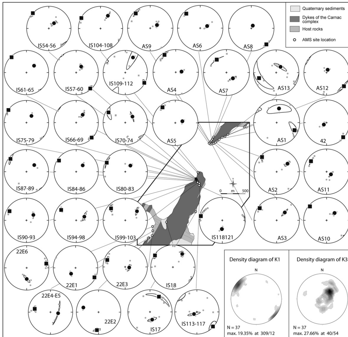
Fig. 6. Equal area projection (lower hemisphere) of the AMS results for each site within the Ile aux Moines and Arradon dykes. AMS site locations within the Ile aux Moines and Arradon dykes are given by small white circles on the map. On the stereoplots, squares and circles are K1 (magnetic lineation) and K3 (pole of magnetic foliation), respectively. Small grey dots and larger black ones represent individual specimen and site-mean direction, respectively. Confidence ellipses at 95% level are drawn around average orientation direction. In the bottom-right corner equal-area projections (lower hemisphere) show the density contours of individual AMS foliation and AMS lineation.
