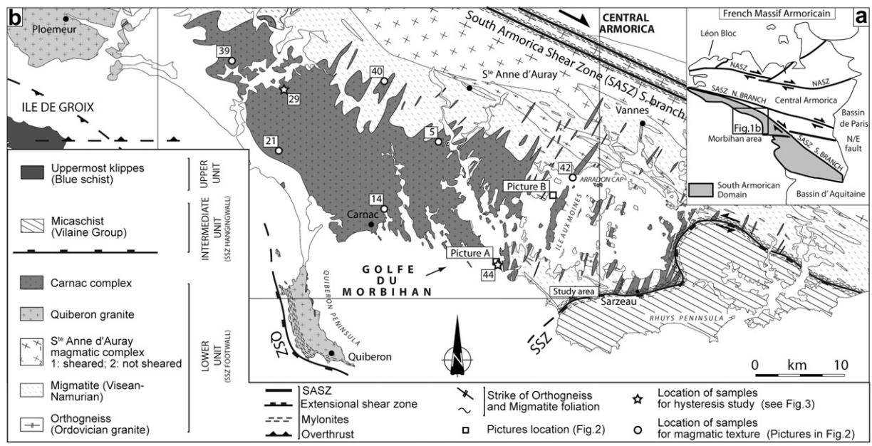
Fig. 1. (a) Simplified map of the Massif Armoricain. NASZ: North Armorican Shear Zone, SASZ: South Armorican Shear Zone, N. Branch: Northern Branch, S. Branch: Southern Branch; (b) Structural map of the Morbihan area in the South Armorican domain (Modified from Turrillot et al., 2009). The main tectonostratigraphic units and their internal features are depicted. The Intermediate and the Lower units are separated by the extensional Sarzeau Shear Zone (SSZ) in the Rhuy Peninsula, and the Quiberon Shear Zone (QSZ) in the Quiberon Peninsula.
