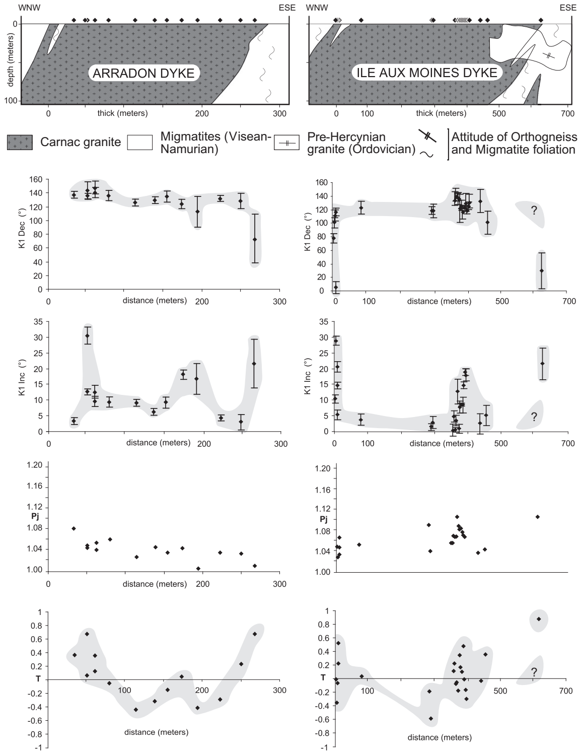
Fig. 7. Cross sections through the Arradon and the Ile aux Moines dykes showing the variations of K1 declination (°), K1 inclination (°), anisotropy degree ( P_j ) and shape parameter (T) across the dykes. Black dots are AMS sites projected on the cross-sections with respect to their distance to the border of the dykes. On the diagrams, the grey surfaces represent the mean variation of the different parameters. The errors bars correspond to the confidence parameter ( \alpha_{95min} ).
