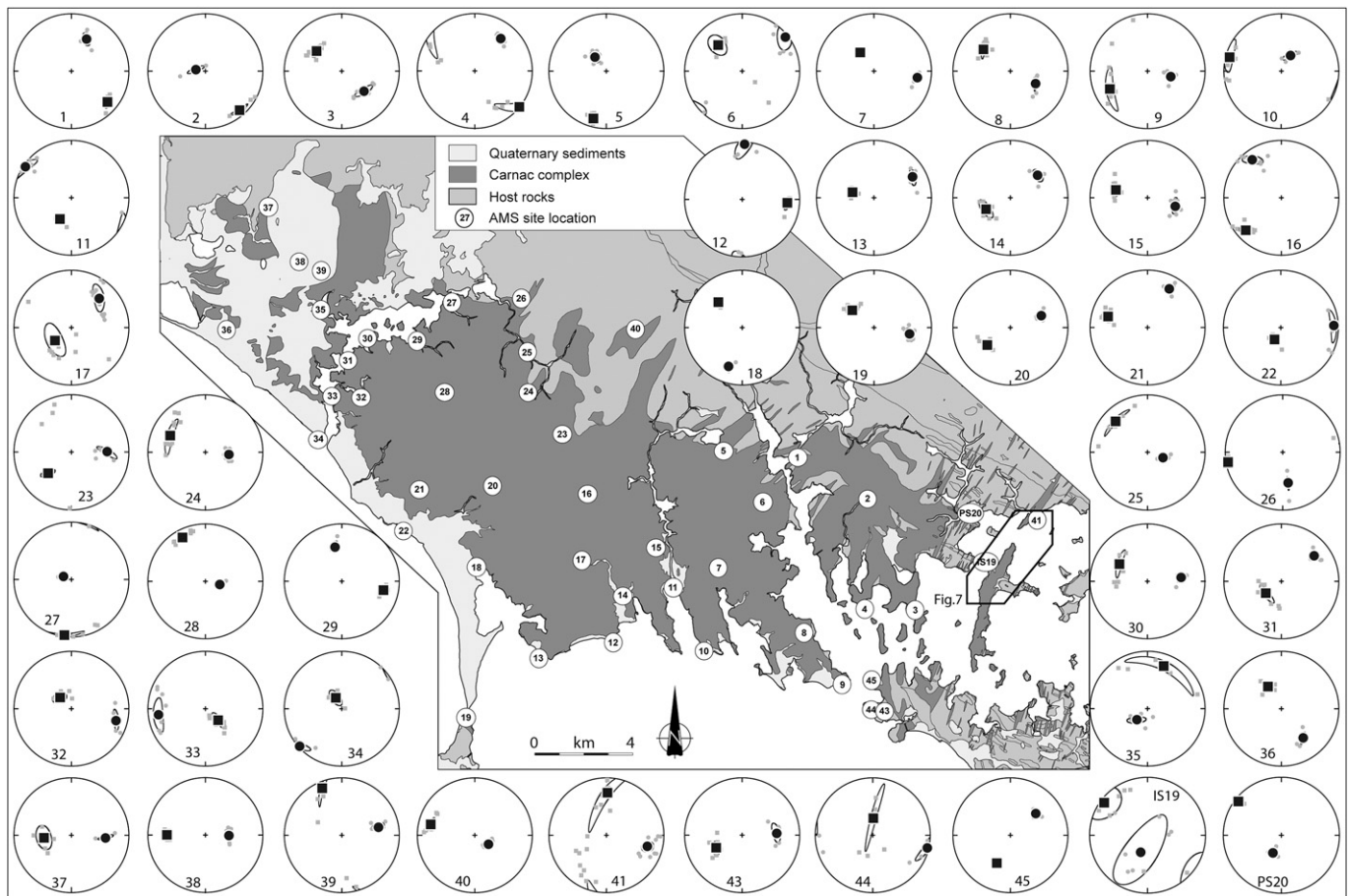
Fig. 4. Equal area projection (lower hemisphere) of the AMS results for each site within the Carnac Complex. On the map, the white circled numbers refer to the AMS sites. On the stereoplots, squares and circles are K1 (magnetic lineation) and K3 (pole of magnetic foliation), respectively. Small grey dots and large black ones represent individual specimens and site-mean direction, respectively. Confidence ellipses at 95% level are drawn around average orientation direction.
