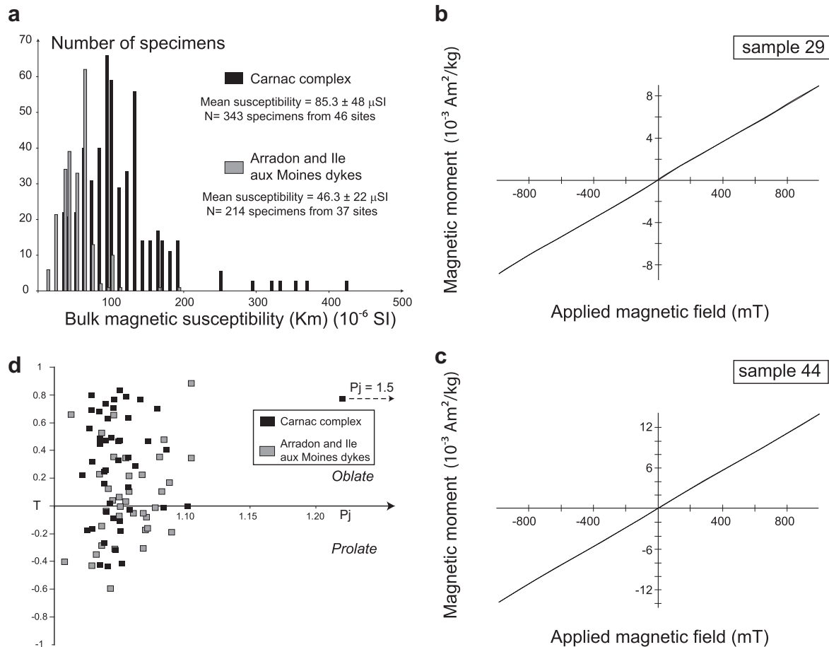
Fig. 3. Information related to the magnetic mineralogy of the entire Carnac Complex and of the dykes. (a) Histogram of the bulk magnetic susceptibility measured from specimens of the Carnac Complex (black) and of the dykes of Ile aux Moines and Arradon (grey); (b) Hysteresis measurements of one specimen from the Carnac pluton (sample 29) (c) Hysteresis measurements of one specimen from a dyke (sample 44). The curves are characteristic of paramagnetic minerals showing linear relationships between the applied magnetic field and the magnetic moment; (d) AMS scalar parameters for each site. Anisotropy degree ( P_j ) vs. shape parameter ( T ). AMS sites in the Carnac Complex are represented by black squares, and AMS sites in the Ile aux Moines and Arradon dykes are represented by grey squares.
