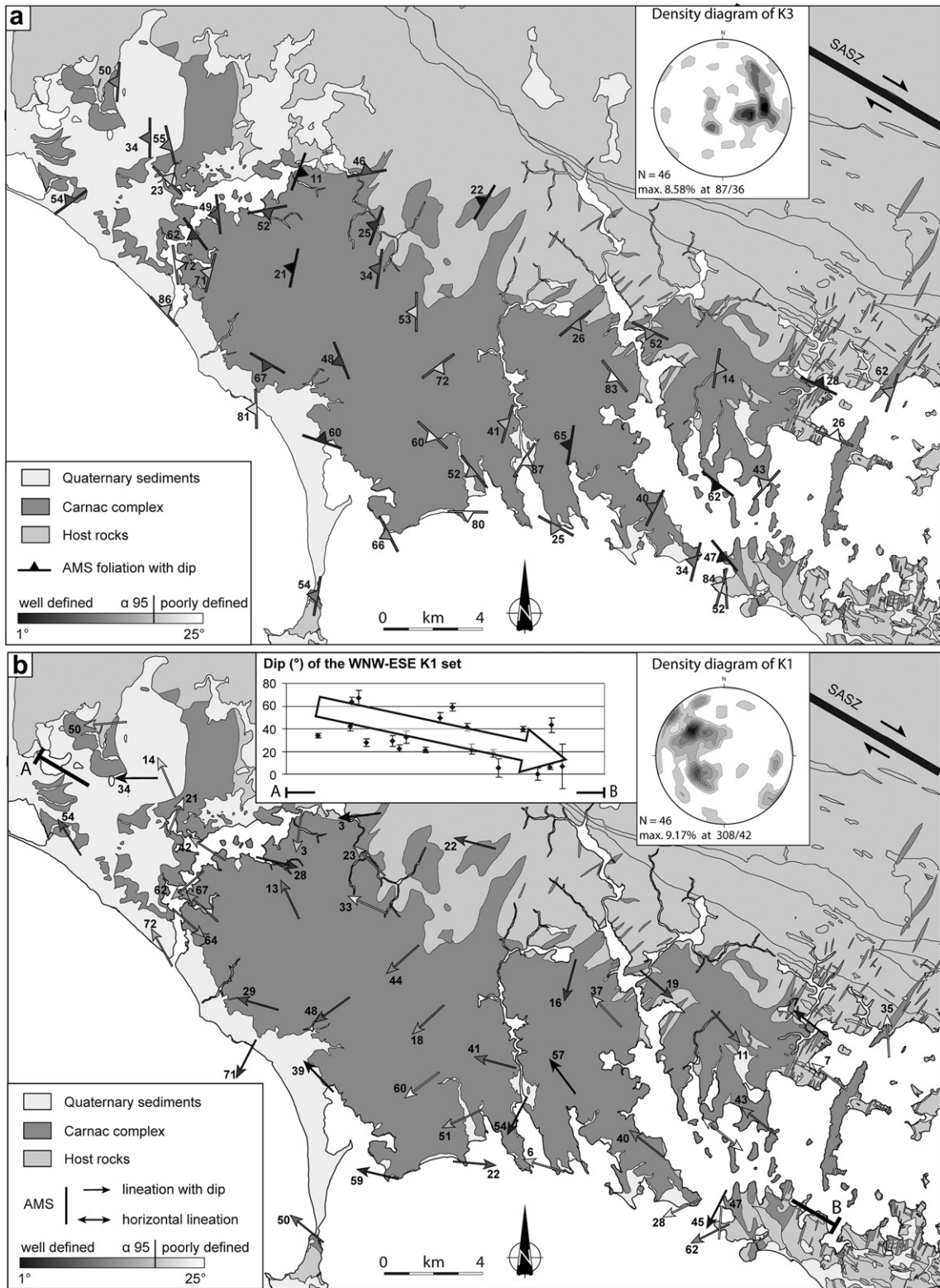
Fig. 5. Magnetic fabric maps of the Carnac Complex. Information on confidence parameter ( \alpha_{95min} ) is given for each magnetic fabric. Equal-area projections (lower hemisphere) show the density contours of individual AMS foliation and AMS lineation. (a) Magnetic foliation; (b) Magnetic lineation. For the WNW-ESE oriented K1 axes, dip variation is given along the A–B section.
