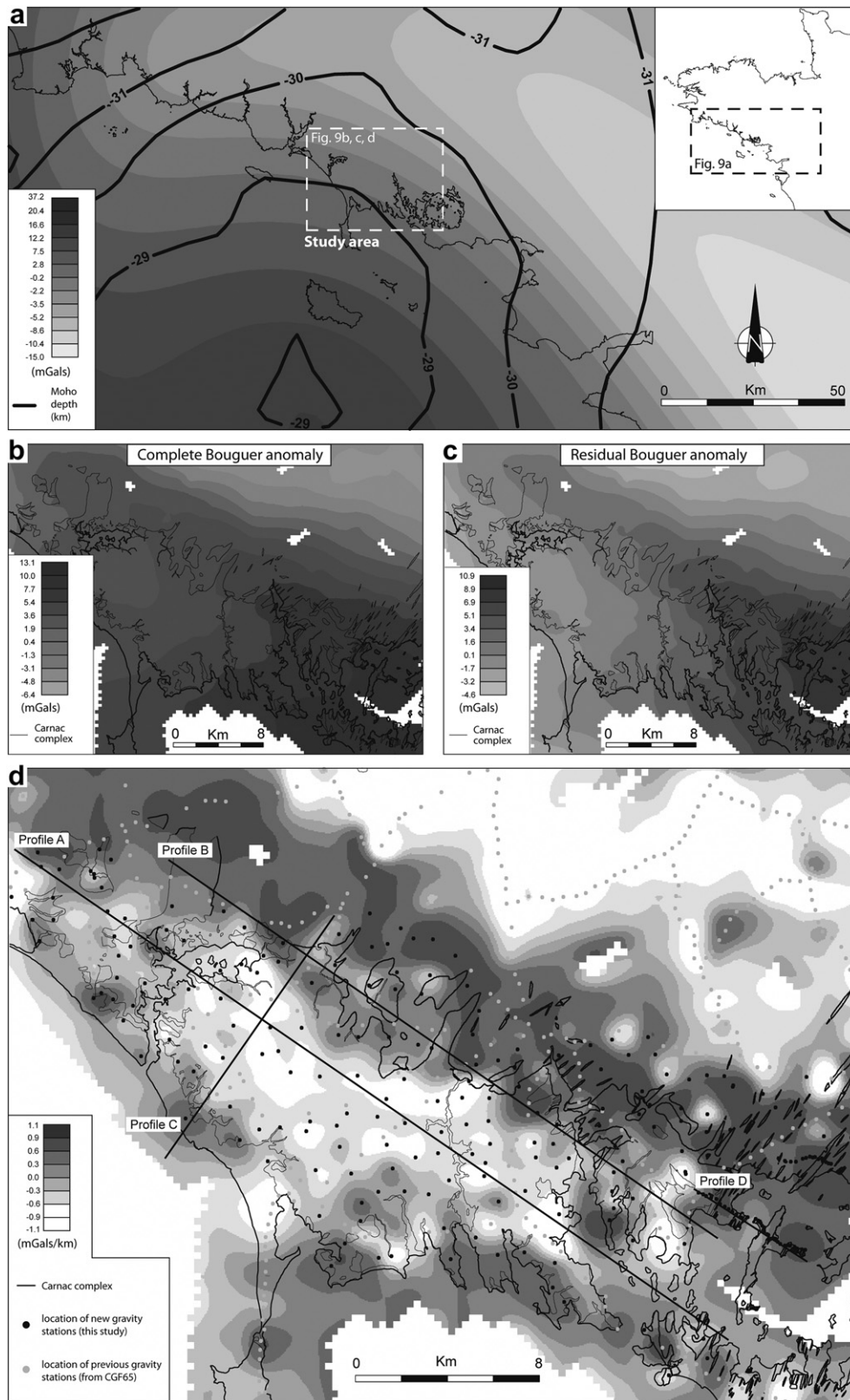
Fig. 8. Main results of the gravity survey. (a) In grey levels, the regional Bouguer anomaly, compared to the regional Moho undulations (black thick lines); (b) Complete Bouguer anomaly of the study area resulting from the combination of our new gravity data and the available gravity data from the BGF French gravity database; (c) resulting residual Bouguer anomaly, mostly influenced by the density heterogeneities located in the first kilometres below the topography. Given are the profile locations of Fig. 9. Black dots correspond to our gravity measurements, grey dots come from the BGF.
