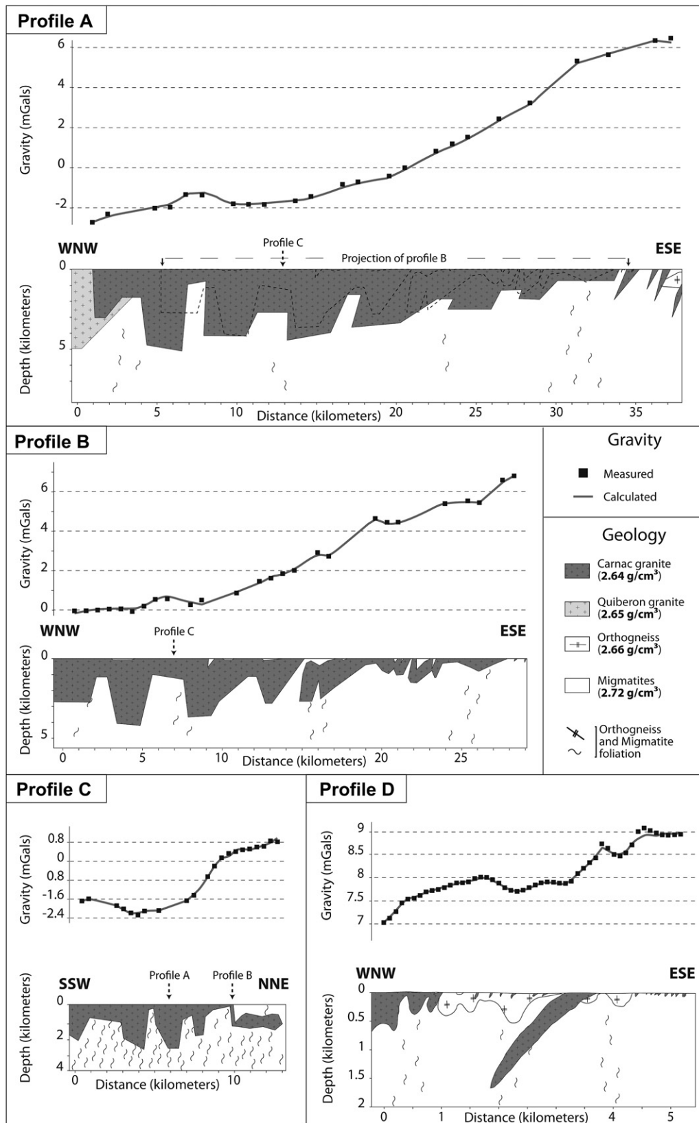
Fig. 9. Forward 2.5D gravity modelling of the Carnac Complex along WNW-ESE and NNE-SSW cross-sections showing the typical geometry of the Carnac Complex with several deep zones interpreted as feeder zones of the pluton. Modelled density values are provided.
