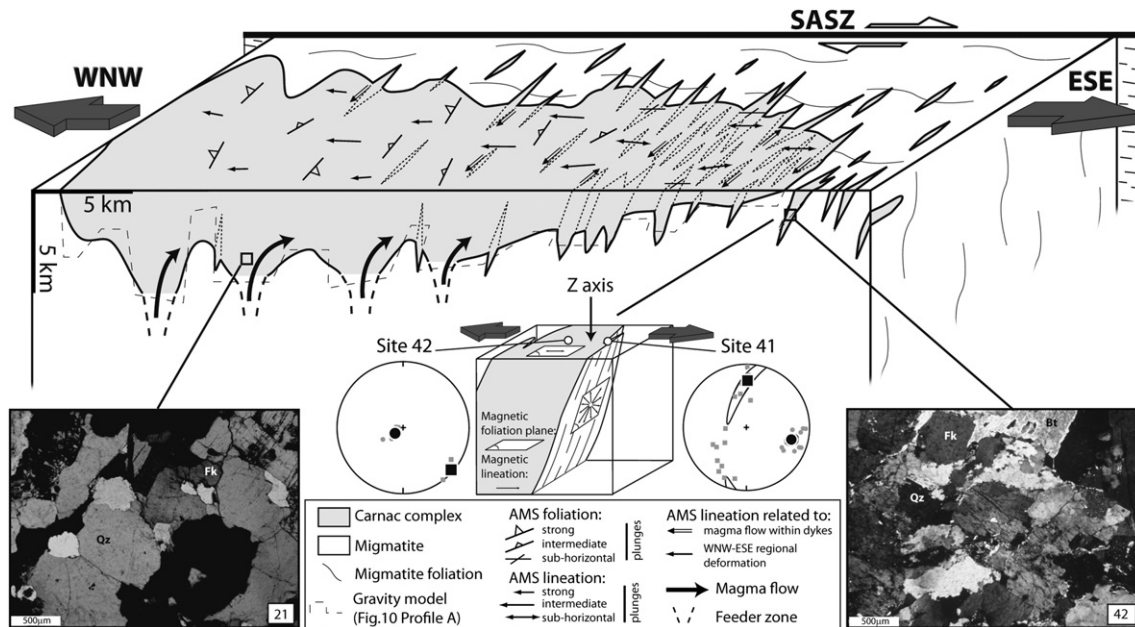
Fig. 10. Three dimensional schematic representation of the Carnac Complex showing the main structural features inferred from AMS and gravity surveys, microstructural observations of the Carnac granite and dyke (numbers refer to AMS sites). The close up is a block diagram illustrating the magnetic fabric within a dyke in which two representative AMS data sites located at the dyke centre and margin are depicted. The NNE-SSW trending indentations of the Carnac pluton are lateral equivalent of the dykes widespread to the east of the Carnac Complex. Thick arrows represent interpreted magma flow during the Carnac pluton emplacement.
